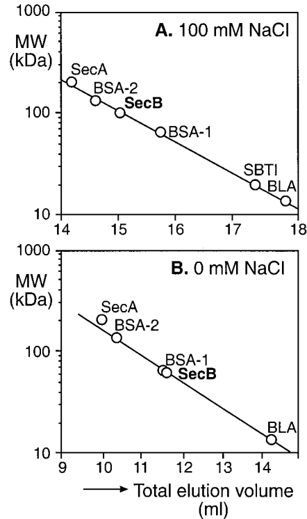
FIGURE 2 Gel filtration analysis of SecB. (A) Elution buffer 10 mM Tris pH 7.5, 100 mM NaCl. (B) Elution buffer 10 mM Tris pH 7.5. BSA-2, dimeric BSA; BSA-1, monomeric BSA.
