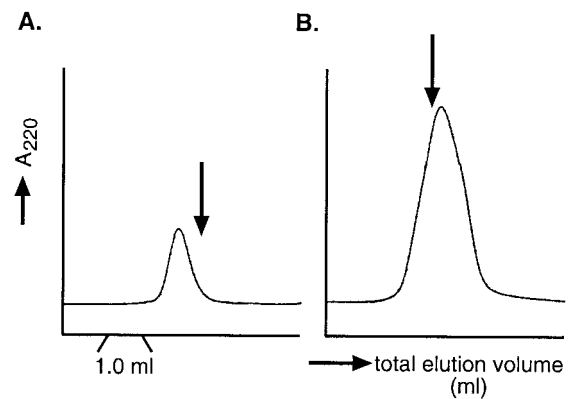
FIGURE 1 Peak profiles in gel filtration chromatographs of 0.2 mg/ml SecB eluted with 10 mM Tris pH 7.5, 100 mM NaCl ( A ); and 0.5 mg/ml SecB eluted with 10 mM Tris pH 7.5 ( B ). The arrows indicate the positions of the peak of monomeric BSA eluted with the corresponding buffers.
