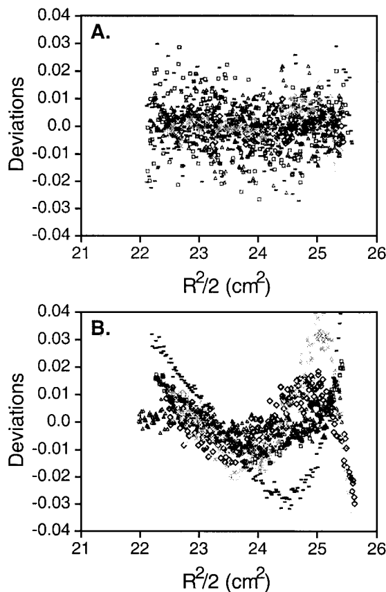
FIGURE 4 Results of sedimentation equilibrium analysis of SecB in 5 mM Tris pH 7.5, 100 mM NaCl (A); and in 5 mM Tris pH 7.5 (B). Shown are the deviations from the fit, where in both panels the symbols correspond to 1.0 mg/ml protein at 11500 rpm (open diamonds); 0.5 mg/ml at 11500 rpm (open squares); 0.2 mg/ml at 11500 (open triangles); 1.0 mg/ml at 15000 rpm (cross); and 0.5 mg/ml at 8500 rpm (minus).
